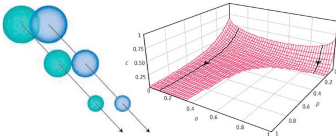
Parting ways. (Left) Sketch of entanglement sudden death, with spheres representing snapshots of the individual qubits moving together in time. The sphere radius indicates the coherence of a single qubit. As the qubits interact with their environment, the spheres naturally shrink smoothly, and in an infinite time each will shrink to the single point that represents its final state. However, entanglement can cease much earlier, as represented here by the time at which the two spheres cease overlapping. (Right) Entanglement sudden death is not limited to the initial states reported by Almeida et al. (6). An independent example (4) is shown here, where concurrence c is plotted vertically against the probability of decay p (which goes to 1 as time goes to infinity) and a , a parameter that selects different initial states. The plot shows an entire family of mixed states, all relaxing under the influence of environmental amplitude noise. In this example, different values of a can correspond to the same initial entanglement c but lead to very different final conditions, some showing entanglement sudden death and some not (black lines).
